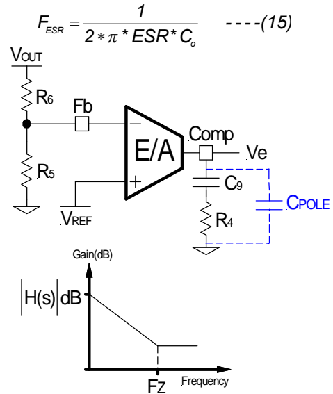
Fig. 19: Typell compensation network and its asymptotic gain plot
